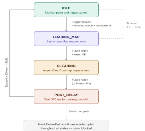
Figure 4.6 Asynchronous tile switch state machine
